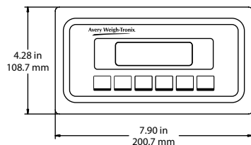
Operator display
